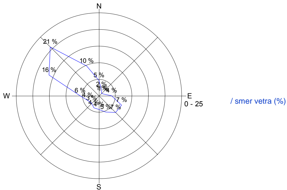
Slika 19: Roža vetrov, december 2017.
