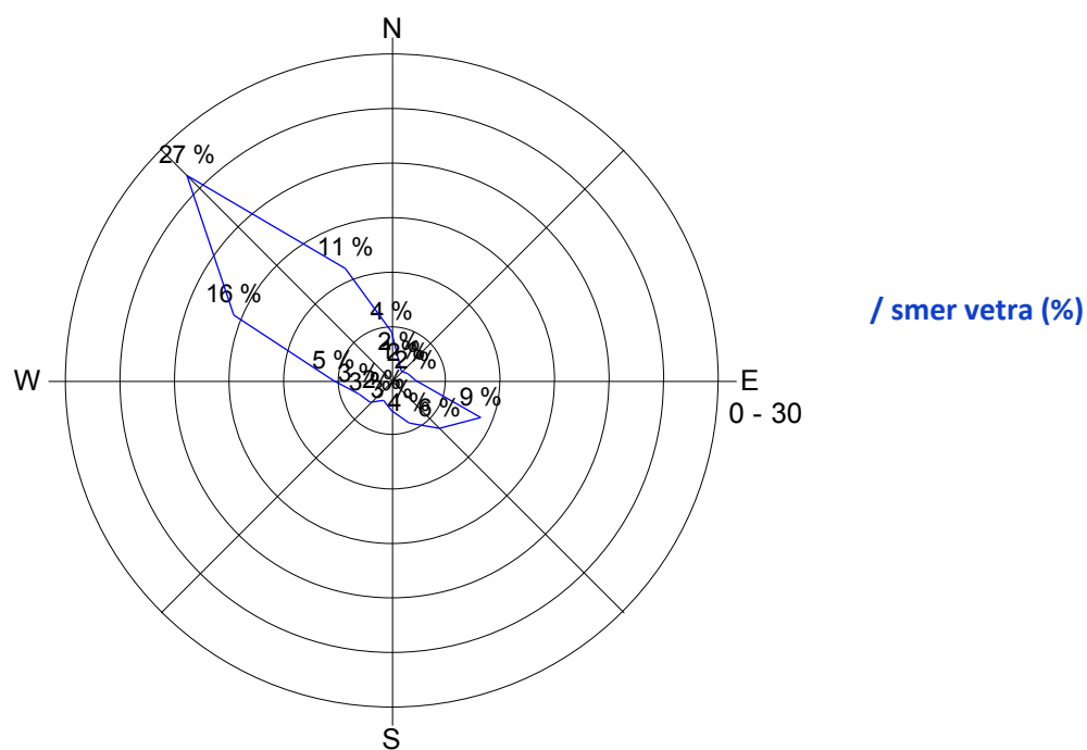
Slika 19: Roža vetrov, december 2015.
