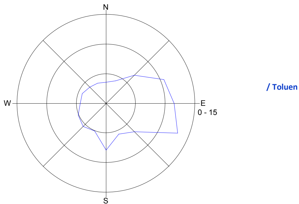
Slika 11: Roža onesnaženost - toluen, december 2014.
